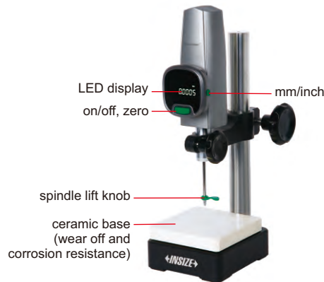
data transmitted to Excel without software; short press the foot switch to transmit data, long press to zero
