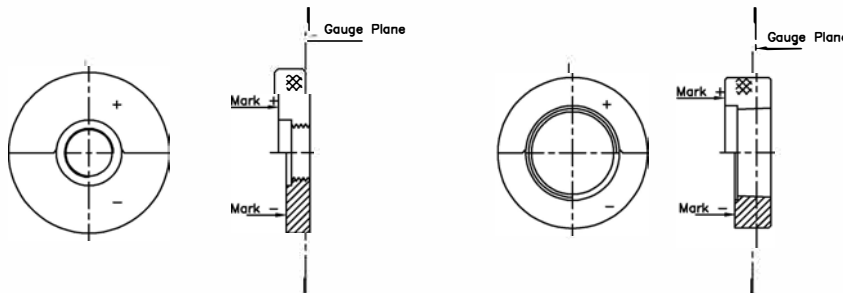
Parallel Full form Thread Ring Gauge. Gauge No.3
