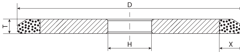
shape 1S1 D \times T \times X \times V \times R \times F \times N \times H
