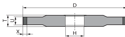
shape 14A1 D \times T \times U \times X \times H
