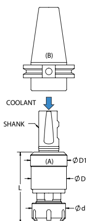
(A) Tap Holder SFTII Cylindrical Shank, ER Collet Chuck, Internal Coolant System
